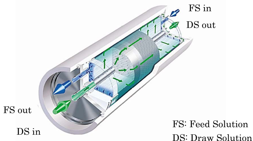
Large-sized hollow fiber FO membrane module (schematic diagram)
